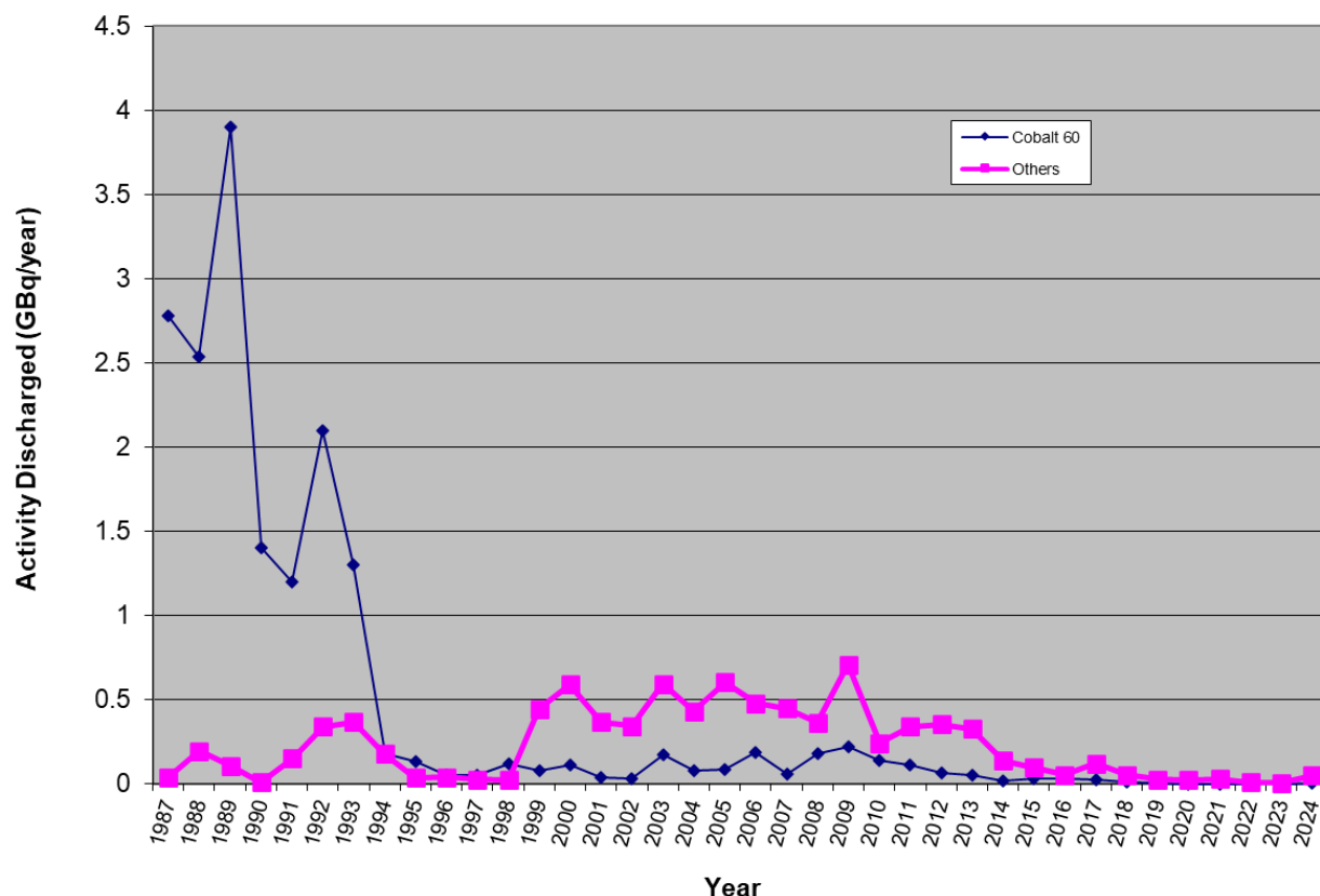
Graph 1 - Cobalt-60 and Other Activity (excluding Tritium) Discharged to the Hamoaze
